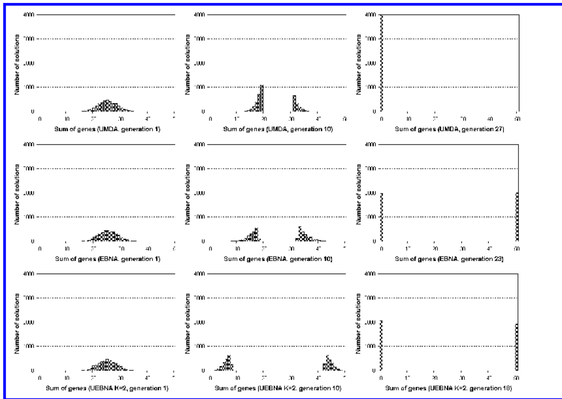
Figure 7: Dynamics of the UMDA (top row), the EBNA (middle row), and the UEBNA (bottom row) until convergence in one run for P_{twomax50} . The horizontal axis of each histogram represents the sum of the genes of a solution, whereas the vertical axis denotes the number of corresponding solutions in the population of different generations.
