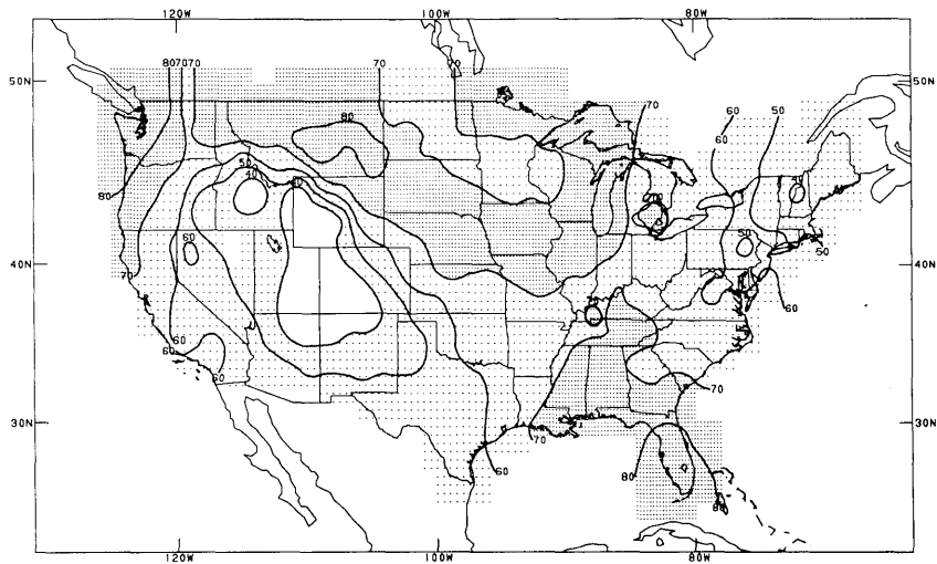
JAN 1950-91 CONSTRUCTED ANALOGUES
