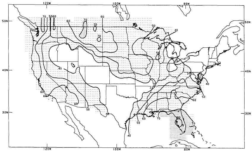
JAN 1950-91 NATURAL ANALOGUES
