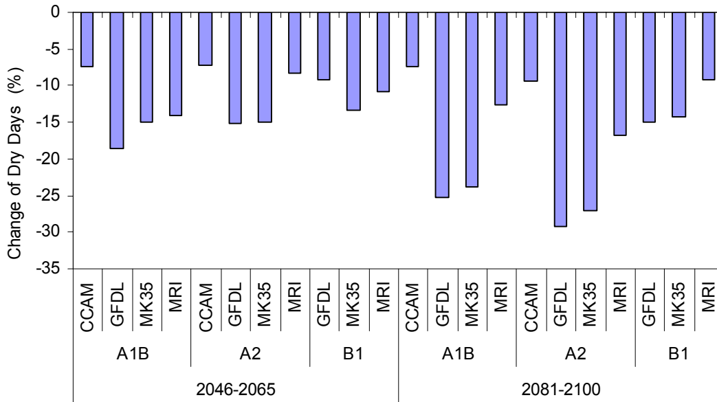
Figure 11. Change in wet day occurrence (%).
