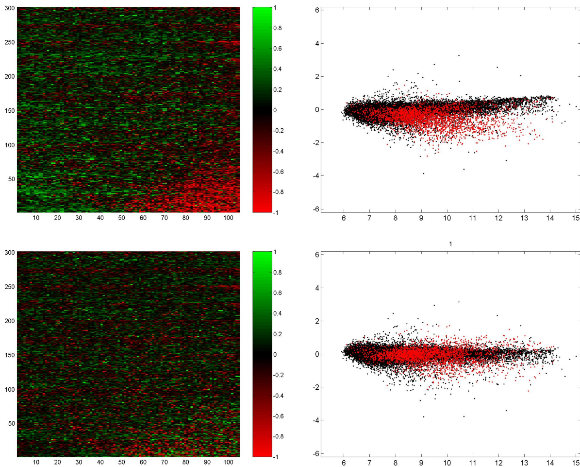
Figure 4. Pre-analysis data transformation using the spatial lowess function. The upper left panel shows log ratios of raw intensity data on a red-green color scale plotted on the spatial coordinates of the array. A bright red corner is apparent on the figure. The upper right panel shows an RI plot of the same data. Spots from the bright corner of the array are highlighted in red. The lower two panels show the array view and RI plots of data after transformations using the spatial lowess smoother.
