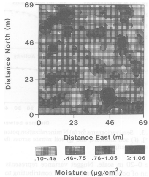
FIG. 7. Isopleths for soil moisture across the study site. Estimation standard deviations for interpolated points range from 0.09 to 0.12 \mu\text{g}/\text{cm}^2 .
