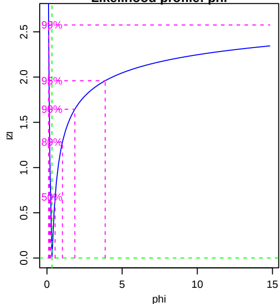
Likelihood profile: phi
