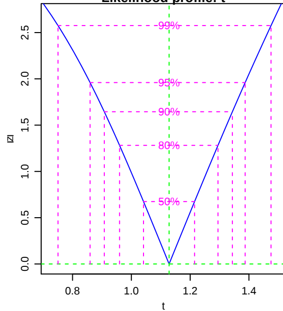
Likelihood profile: t
