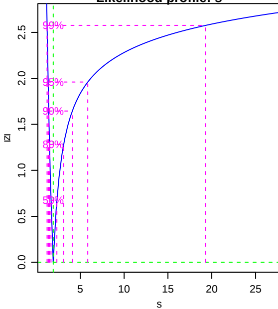
Likelihood profile: s
